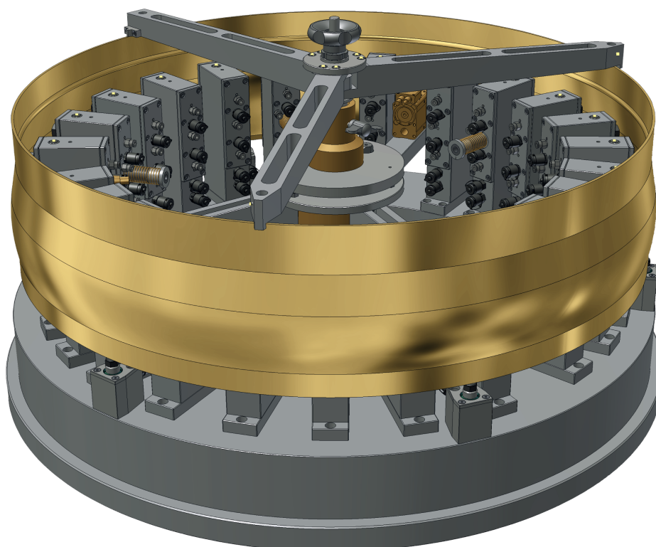
Fixture with jet engine ring shaped component.
