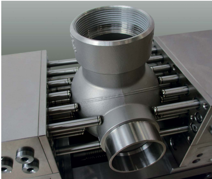
KOSTYRKA® pin jaws on a vice.
