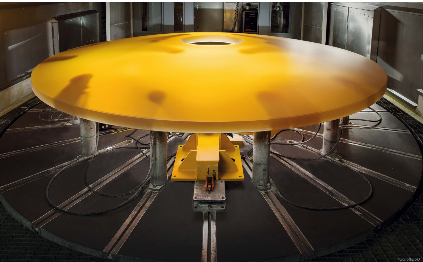
Fixture with mirror blank inside the grinding machine.
