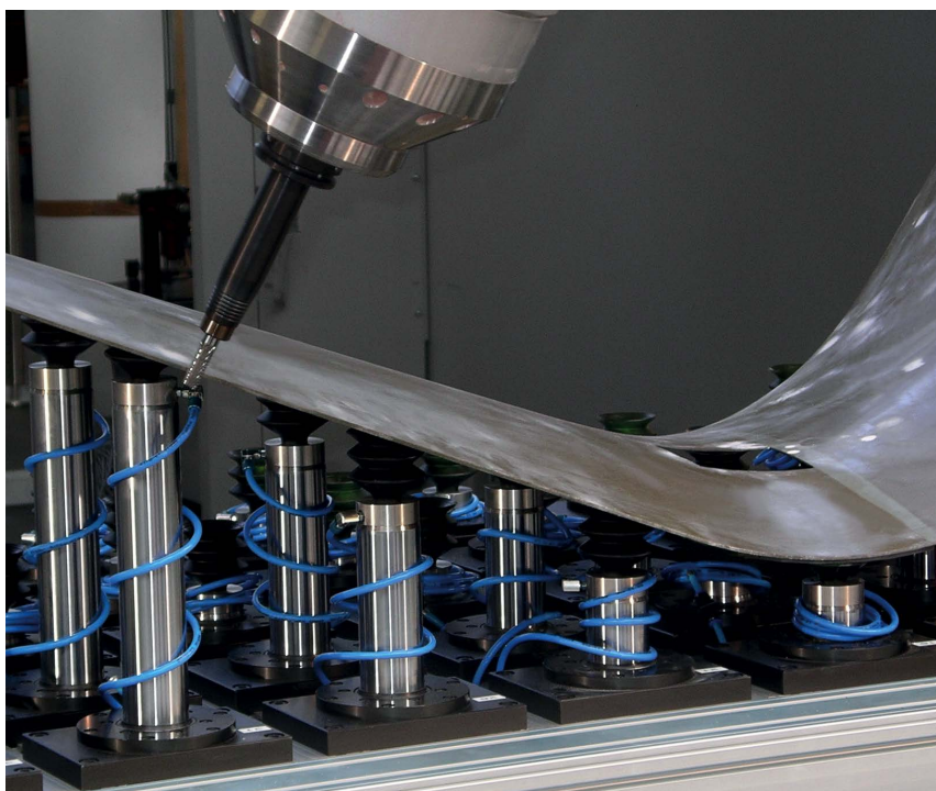
Pin system with vacuum cups.
