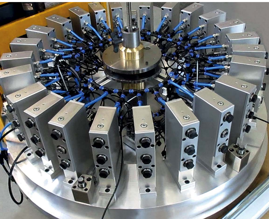
Fixture without component.
